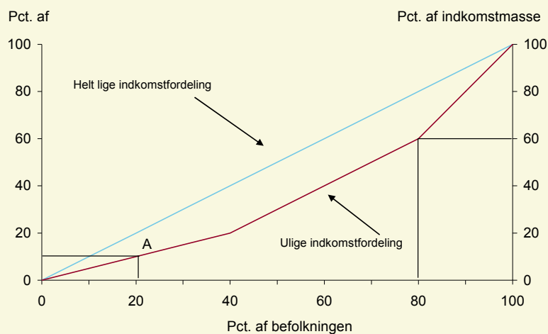
Figur 10 Gini-koefficient
